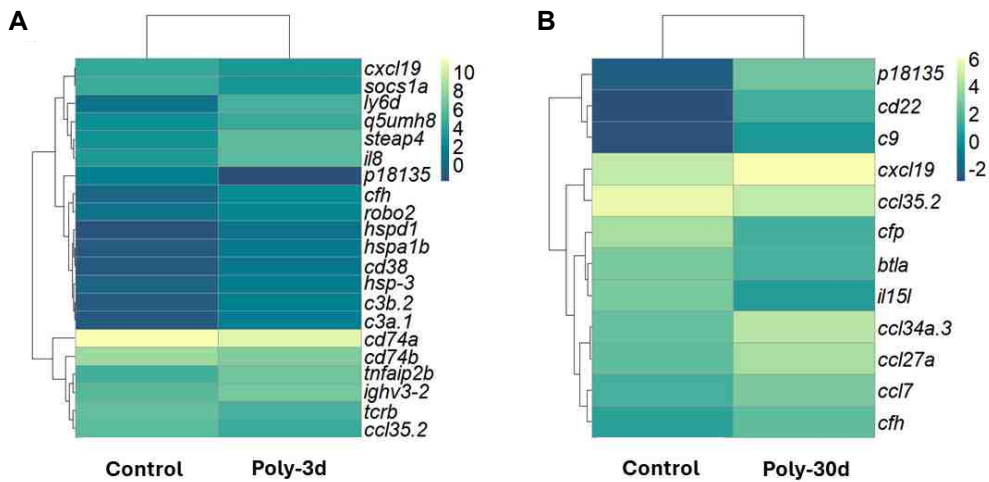
Fig. 1. Heatmaps of selected immune-related DEGs in kidney of olive flounder after Poly (I:C) injection. (A) Expression levels of Immune-related DEGs at day 3 post Poly (I:C) injection. (B) Expression levels of Immune-related DEGs at day 30 post Poly (I:C) injection. Based on FPKM values, Log 2 -transformed gene expression levels are shown in a gradient color scheme in each row.
